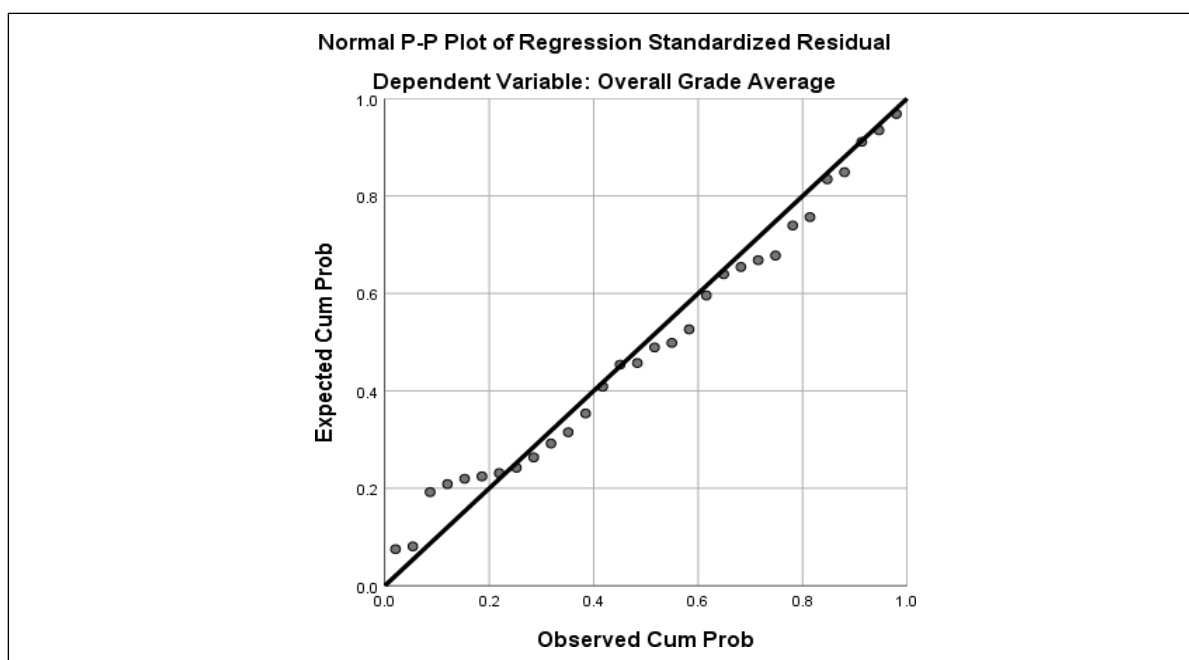
Figure 1. Normal P-P (Probability-Probability) Plot
