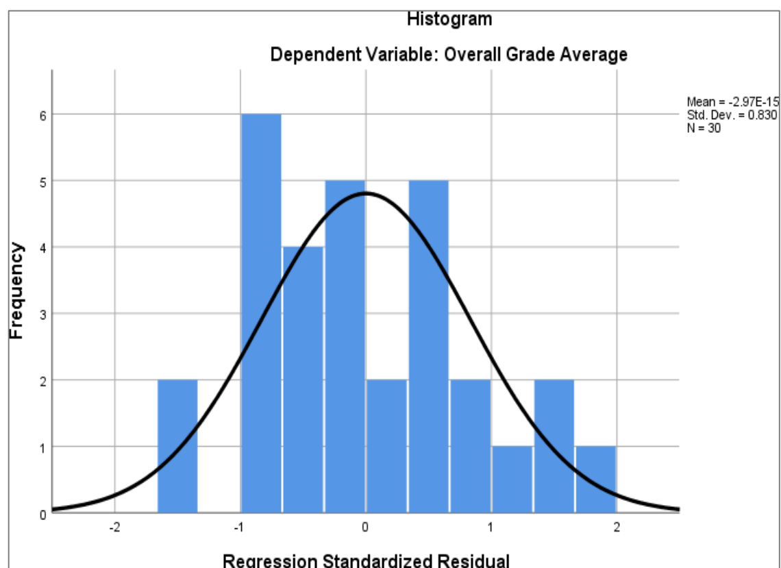
Figure 2. Histogram of Regression Standardized Residuals
