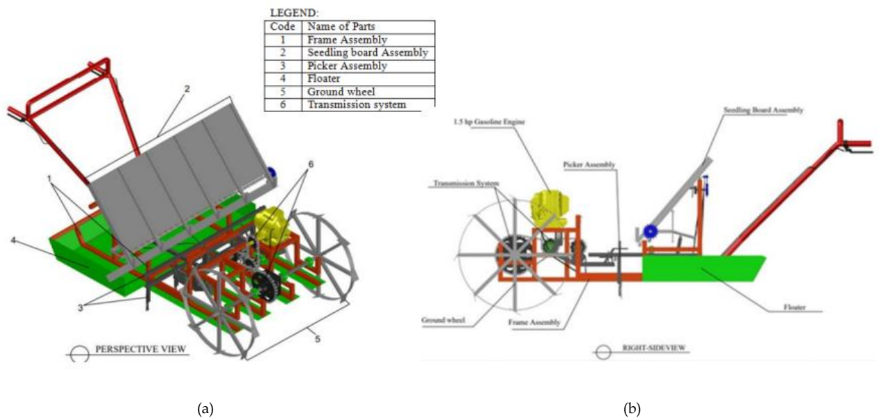
Figure 1. Component parts of the self-propelled mechanical rice transplanter (a) perspective view and (b) right side view.
